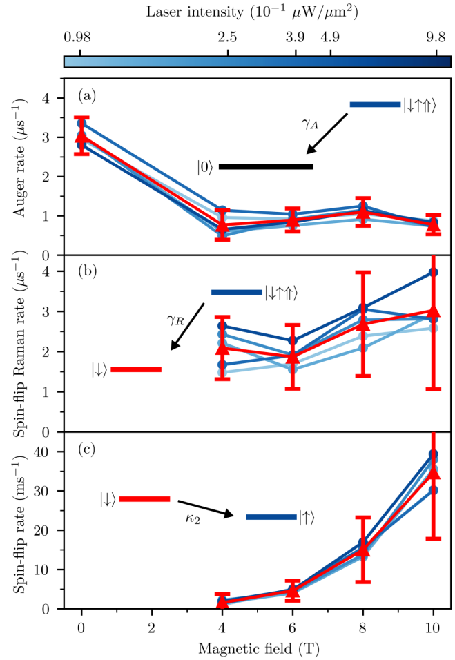
FIG. 4. Magnetic field dependence of the Auger rate (a), spin-flip Raman rate (b), and spin-flip rate (c) for different laser intensities (blue shades, circles), obtained from fits of the numerical solution of Eq. (2). The average rates over all laser intensities for each magnetic field are shown in red triangles. At 0 T, the trion transition degenerates, and we are unable to extract spin-flip nor spin-flip Raman processes with our method.
